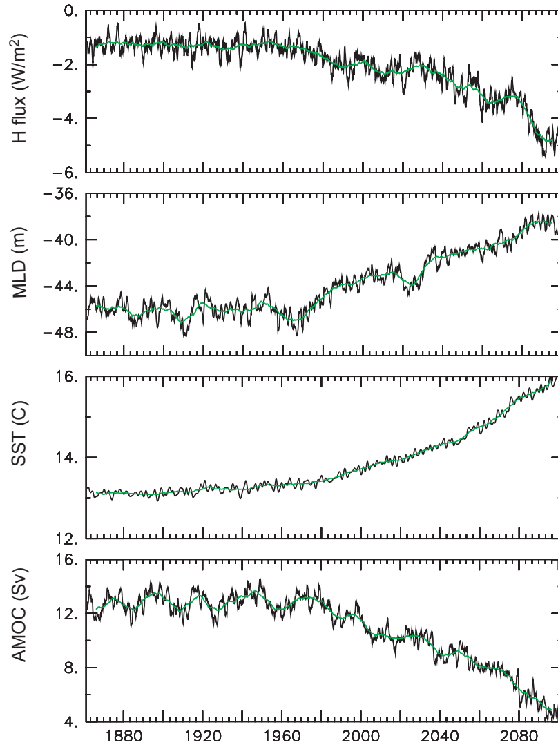
Figure 3.2 — Time series of global heat flux ( \text{W/m}^2 ), Mixed Layer Depth (m), and intensity of the Atlantic Meridional Overturning Circulation (Sverdrup, 10^6 \text{ m}^3/\text{s} ) for the \text{CO}_2 -climate run. Negative values mean fluxes towards the ocean. The time series are deseasonalized (black line). The decadal variability (mean over 10 years) is overlayed, green line.
