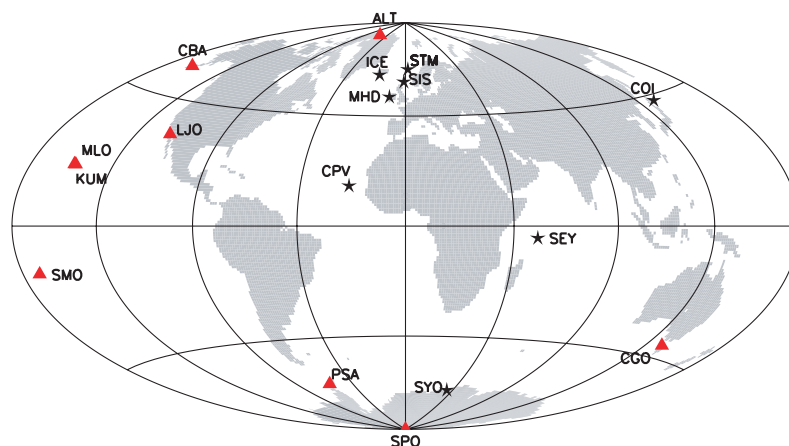
Figure 3.1 — Locations of the stations considered in this study. The stations from the Scripps sampling network used to compare the model results are the in red. Alert, Canada (ALT); Cape Grim, Tasmania (CGO); Cold Bay, Alaska (CBA); Cape Oshi Ishi, Japan (COL); Cape Verde (CPV); Heimaey, Island (ICE); Kumukahi, Hawaii (KUM); La Jolla, California (LJO); Mauna Loa (MLO), Hawaii; Mace Head, Ireland (MHD); Palmer Station, Antarctica (PSA); Samoa, American Samoa (SMO); Seychelles (SEY); Shetland, UK (SIS); South Pole (SPO); Station M, Norwegian Sea (STM); Syowa, Antarctica (SYO).
