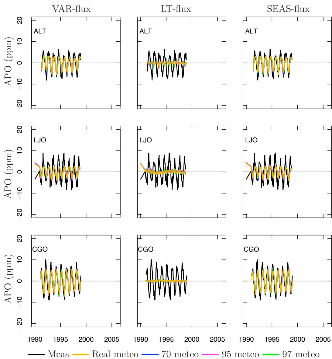
Figure 4.20 — APO Anomalies resulting from the transport of the three MIT- fluxes with different meteorological fields. The stations are displayed in latitudinal bands.
