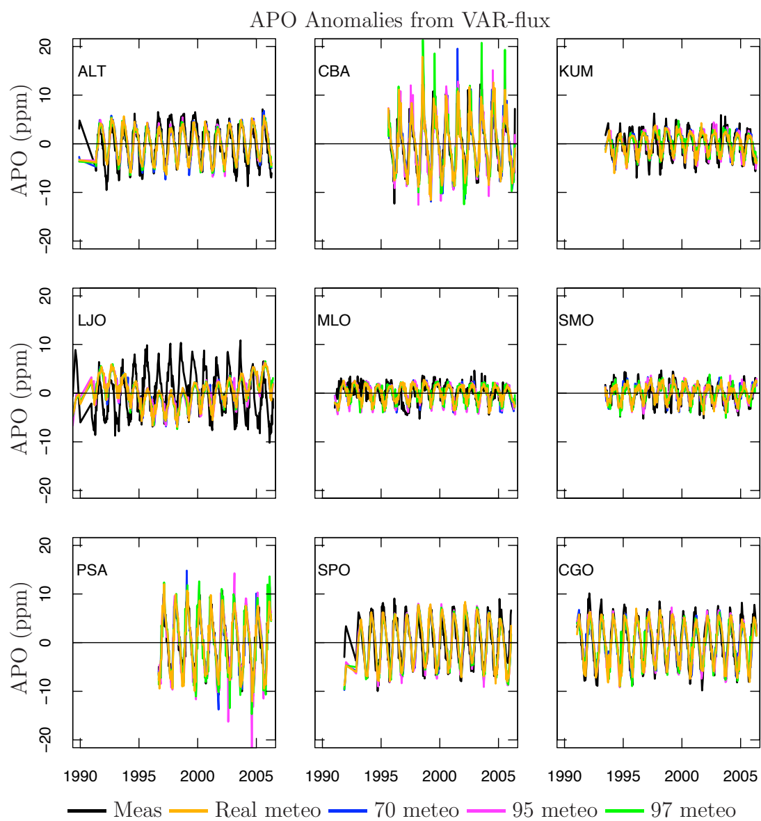
Figure 4.5 — APO Anomalies resulting from the transport of VAR-flux with different meteorological fields. The stations are displayed in latitudinal bands from North to South.
