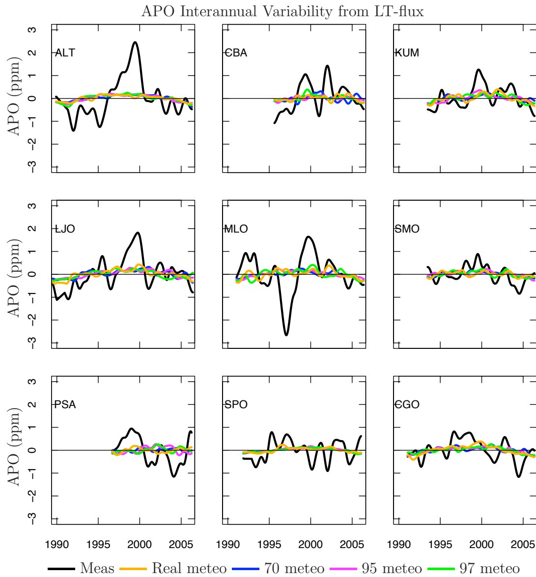
Figure 4.15 — APO Interannual Variability resulting from the transport of LT-flux with different meteorological fields.
