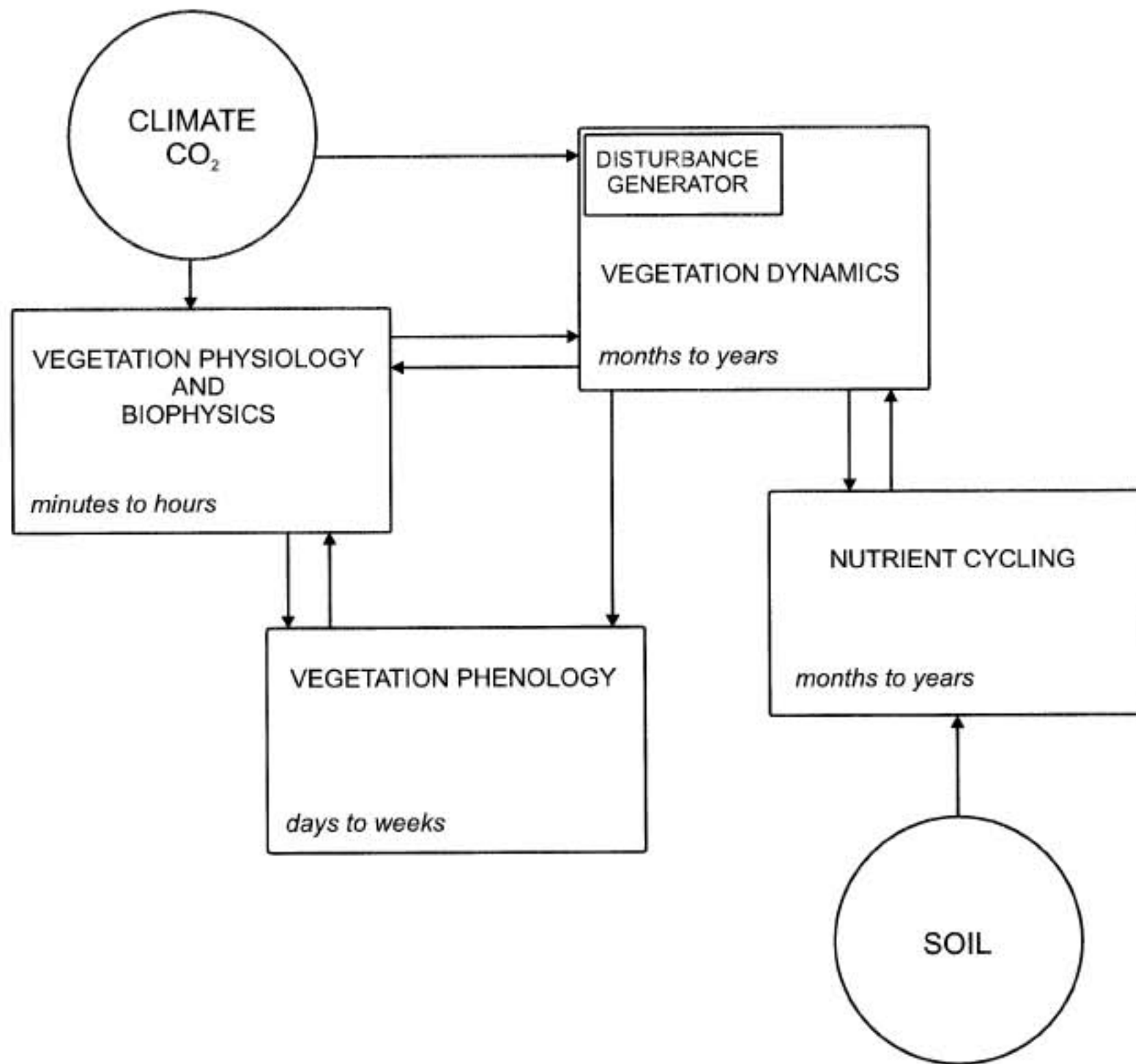
Fig. 1 Modular structure of a generic dynamic global vegetation model (DGVM) as employed with various modifications by the six models. The time steps of the modules are shown in italics. From Cramer et al. (2001), Global Change Biology 7, 357-373
